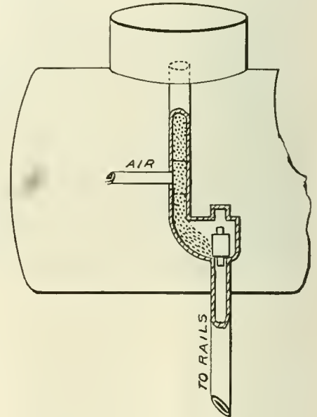
WATTERS' CONVERTIBLE SANDER.
